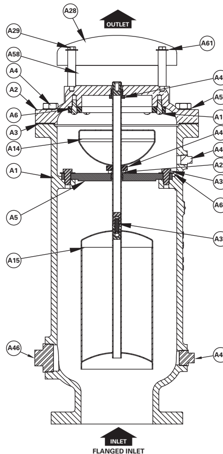
4-14" Valves
