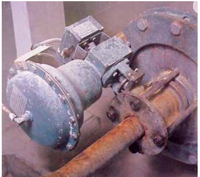
DeZURIK RCV Rotary Control Valve in abrasive kaolin clay slurry application.
